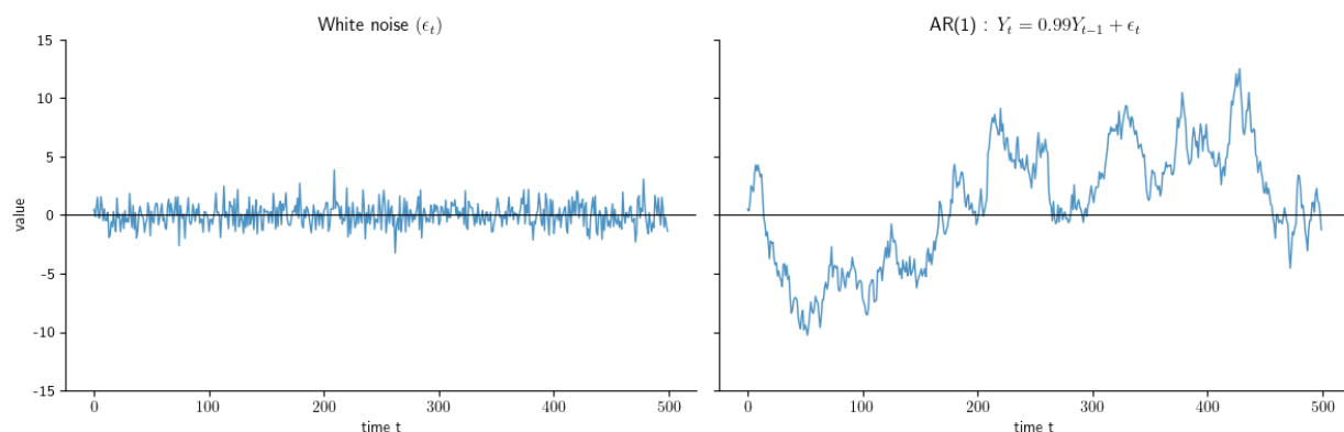
Figure 1.17: Unlike MA since AR looks at all of the past, it blows up when we give more and more importance to the past; more pecisely as |\phi_1| approaches 1.
