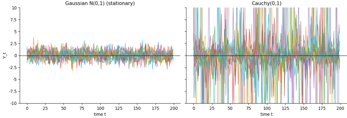
Figure 1.5: A typical process with finite variance (left) and one with infinite variance (right).
